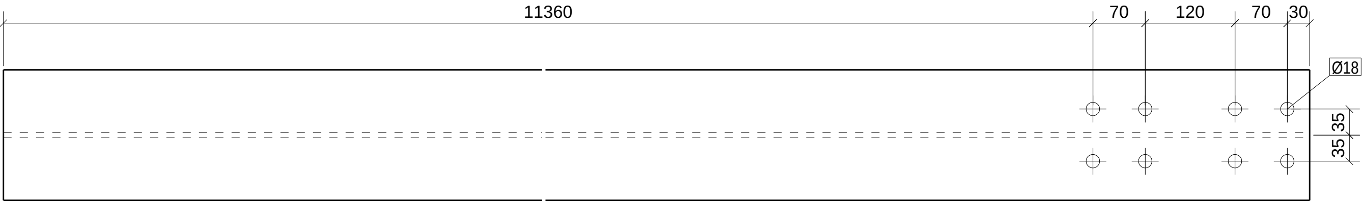
TOP VIEW
